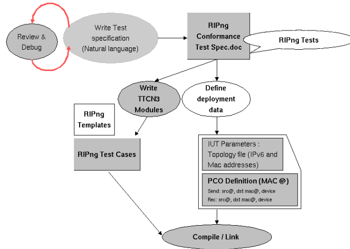
Fig. 3. TTCN-3 based initial approach of test specification
